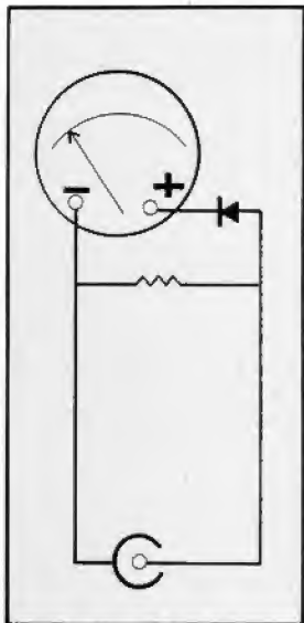
Figure 2: Circuit diagram of the azimuth tester
